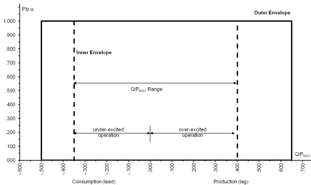
Figure 9 - P - Q/P_{\max} -profile of a Power Park Module. The diagram represents boundaries of a P - Q/P_{\max} -profile at the Connection Point by the Active Power, expressed by the ratio of its actual value and the Maximum Capacity in per unit, against the ratio of the Reactive Power ( Q ) and the Maximum Capacity ( P_{\max} ). The position, size and shape of the inner envelope are indicative.
