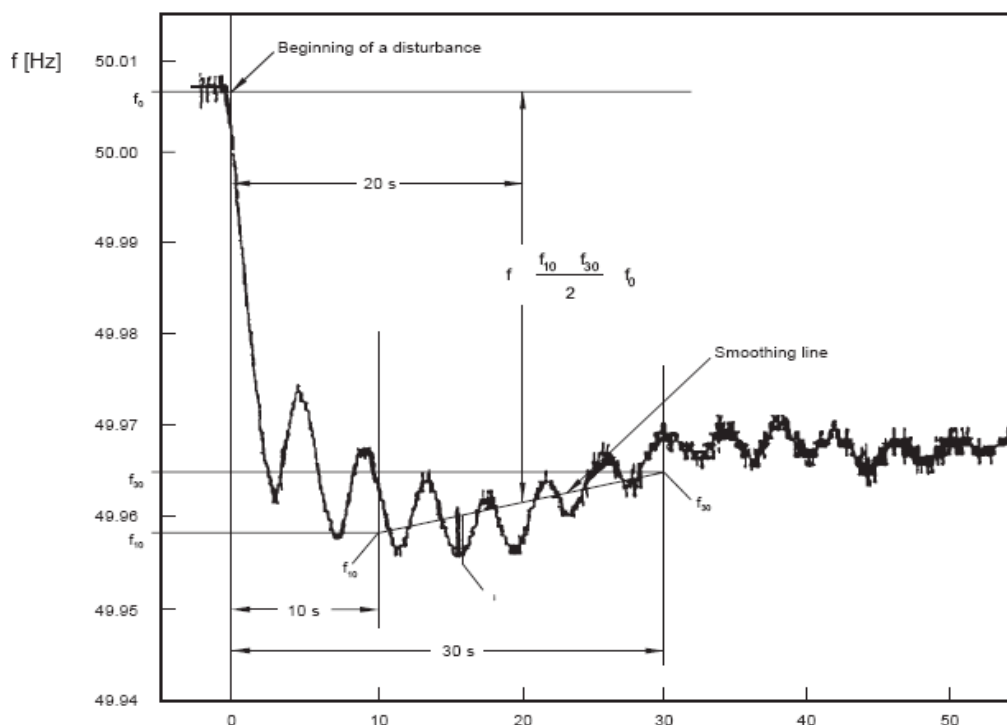
Figure 3: Transient and stead state characteristic 1
