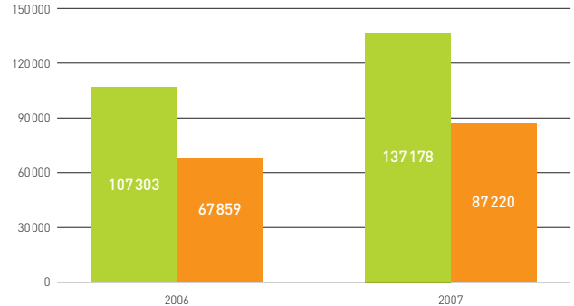
UCTE Production other renewable energy sources including wind power in the year 2006 and 2007 in GWh 1
