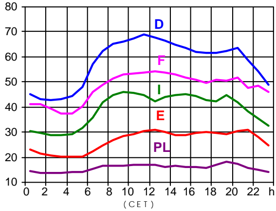
17.09.2003 (in GW)
