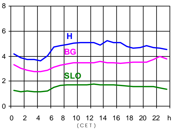
18.06.2003 (in GW)
