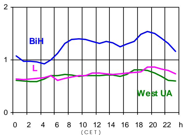
19.03.2003 (in GW)
