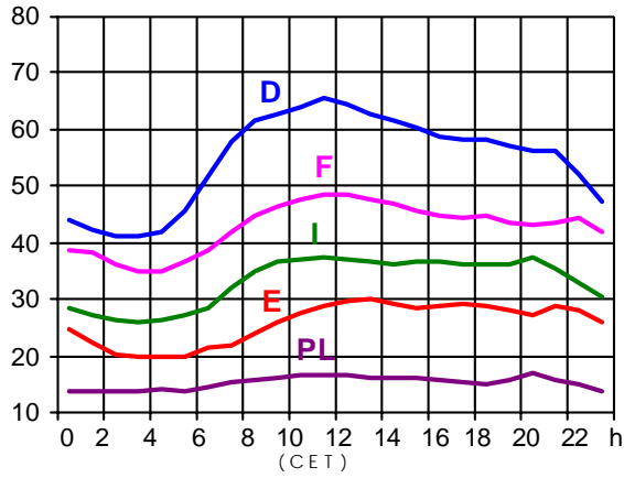
20.08.2003 (in GW)
