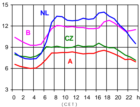
17.12.2003 (in GW)
