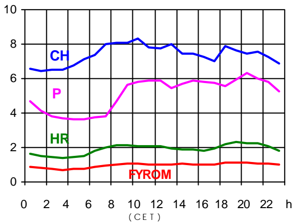
19.03.2003 (in GW)
