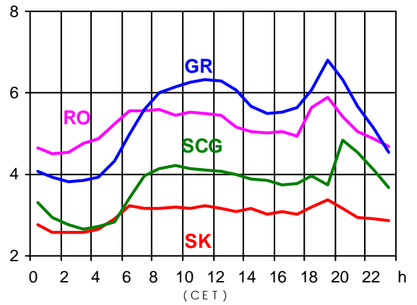
17.09.2003 (in GW)
