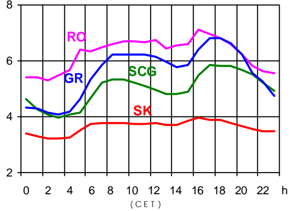
19.11.2003 (in GW)
