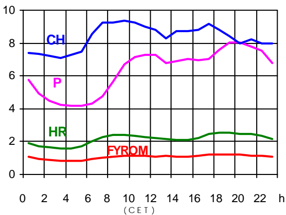
15.01.2003 (in GW)
