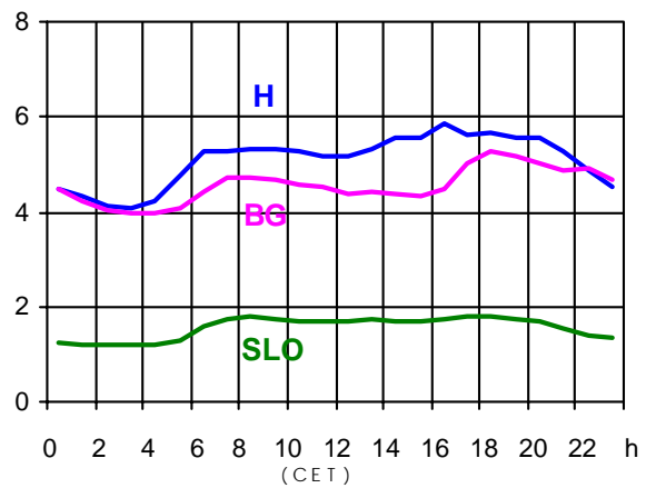
19.11.2003 (in GW)
