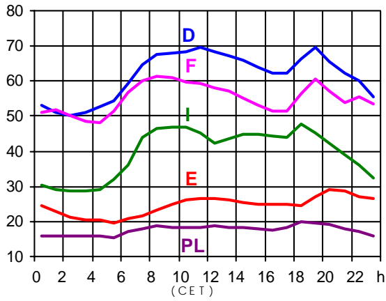
19.03.2003 (in GW)
