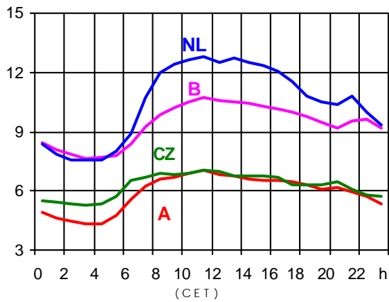
20.08.2003 (in GW)
