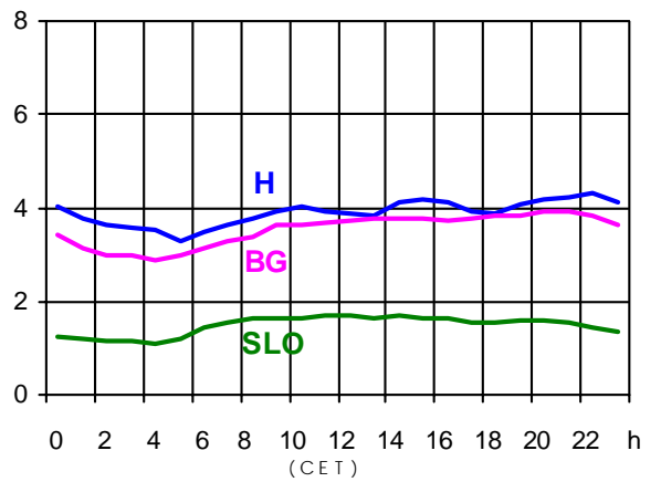
20.08.2003 (in GW)
