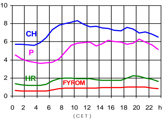
15.10.2003 (in GW)
