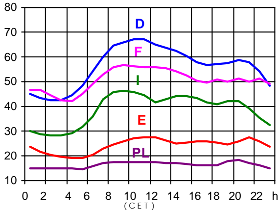
16.04.2003 (in GW)
