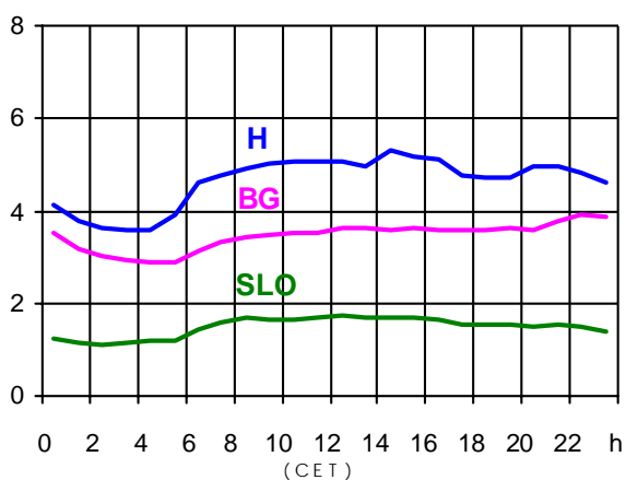
16.07.2003 (in GW)
