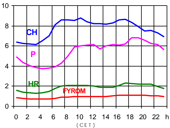
19.11.2003 (in GW)
