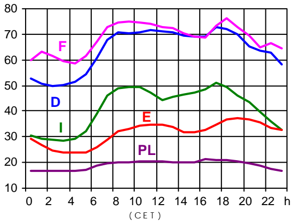
15.01.2003 (in GW)
