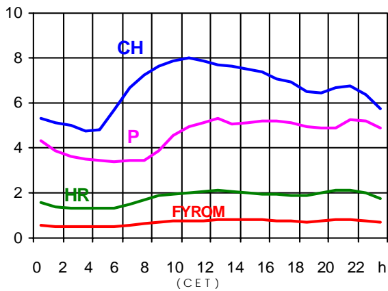
20.08.2003 (in GW)
