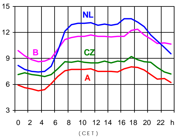
19.11.2003 (in GW)
