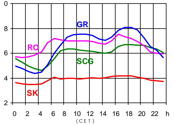
17.12.2003 (in GW)
