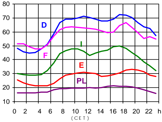
19.11.2003 (in GW)
