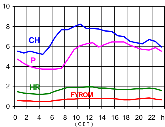
18.06.2003 (in GW)
