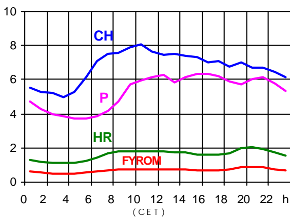
17.09.2003 (in GW)
