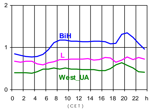
17.09.2003 (in GW)
