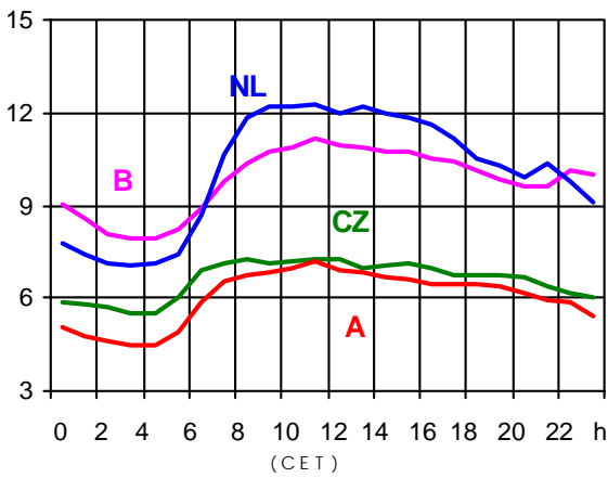
21.05.2003 (in GW)
