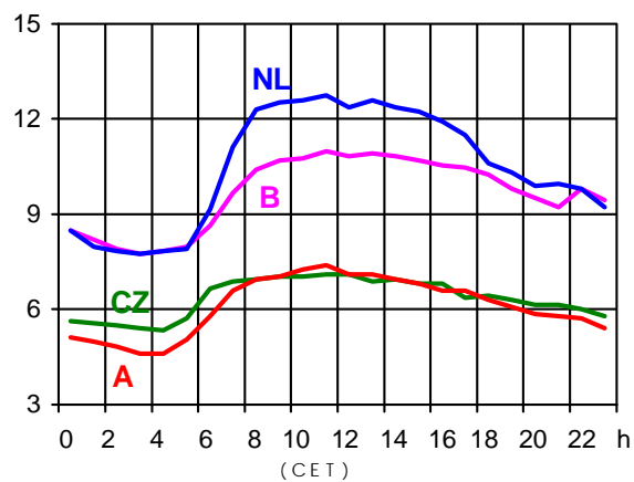
18.06.2003 (in GW)
