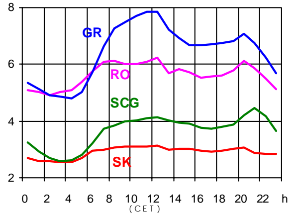
18.06.2003 (in GW)
