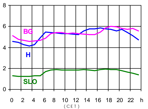
17.12.2003 (in GW)
