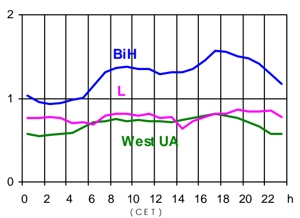
19.11.2003 (in GW)
