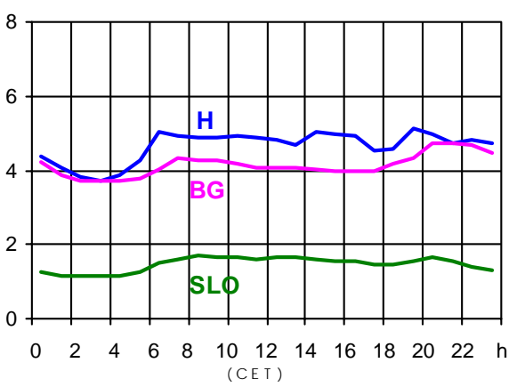
16.04.2003 (in GW)
