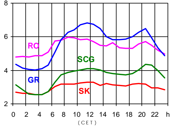
21.05.2003 (in GW)
