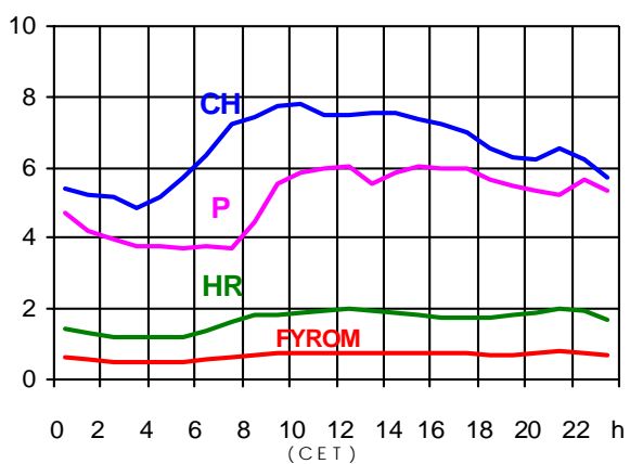
16.07.2003 (in GW)
