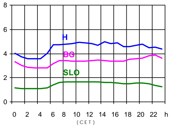
21.05.2003 (in GW)
