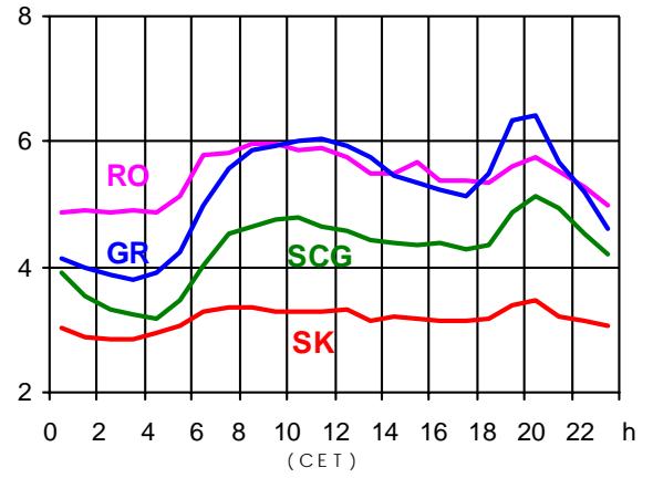
16.04.2003 (in GW)
