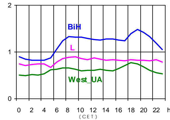
15.10.2003 (in GW)
