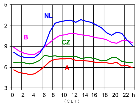
16.04.2003 (in GW)
