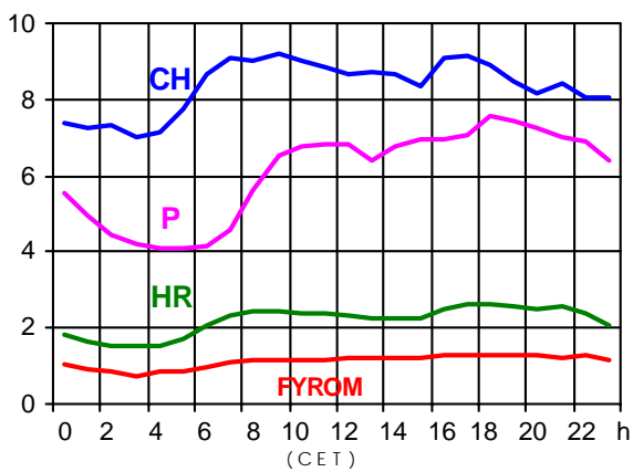
17.12.2003 (in GW)
