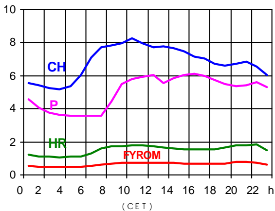
21.05.2003 (in GW)
