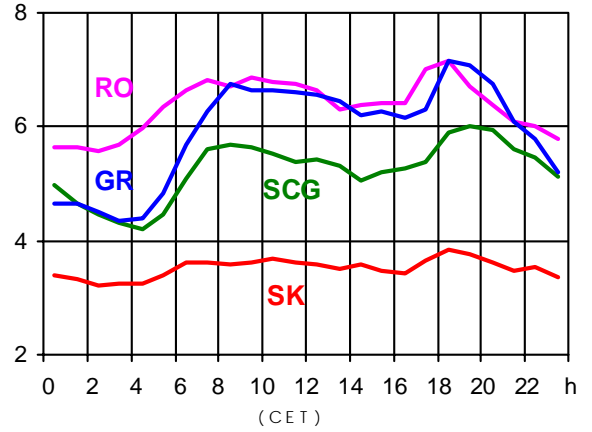
19.03.2003 (in GW)
