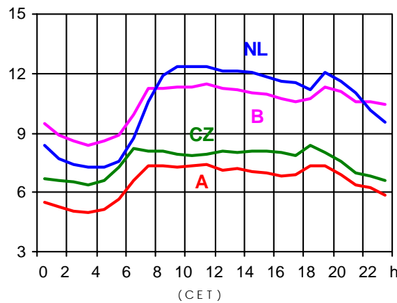
15.10.2003 (in GW)
