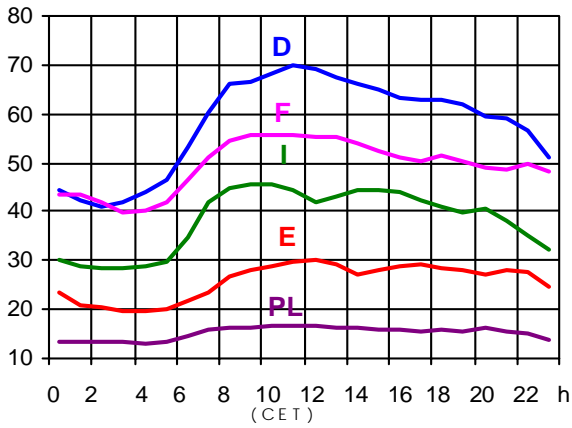
21.05.2003 (in GW)
