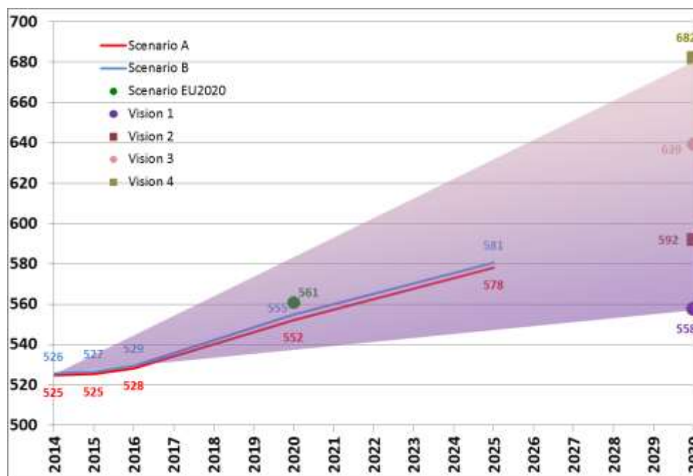
Figure 1.1a. Load (all Scenarios, January; GW)
