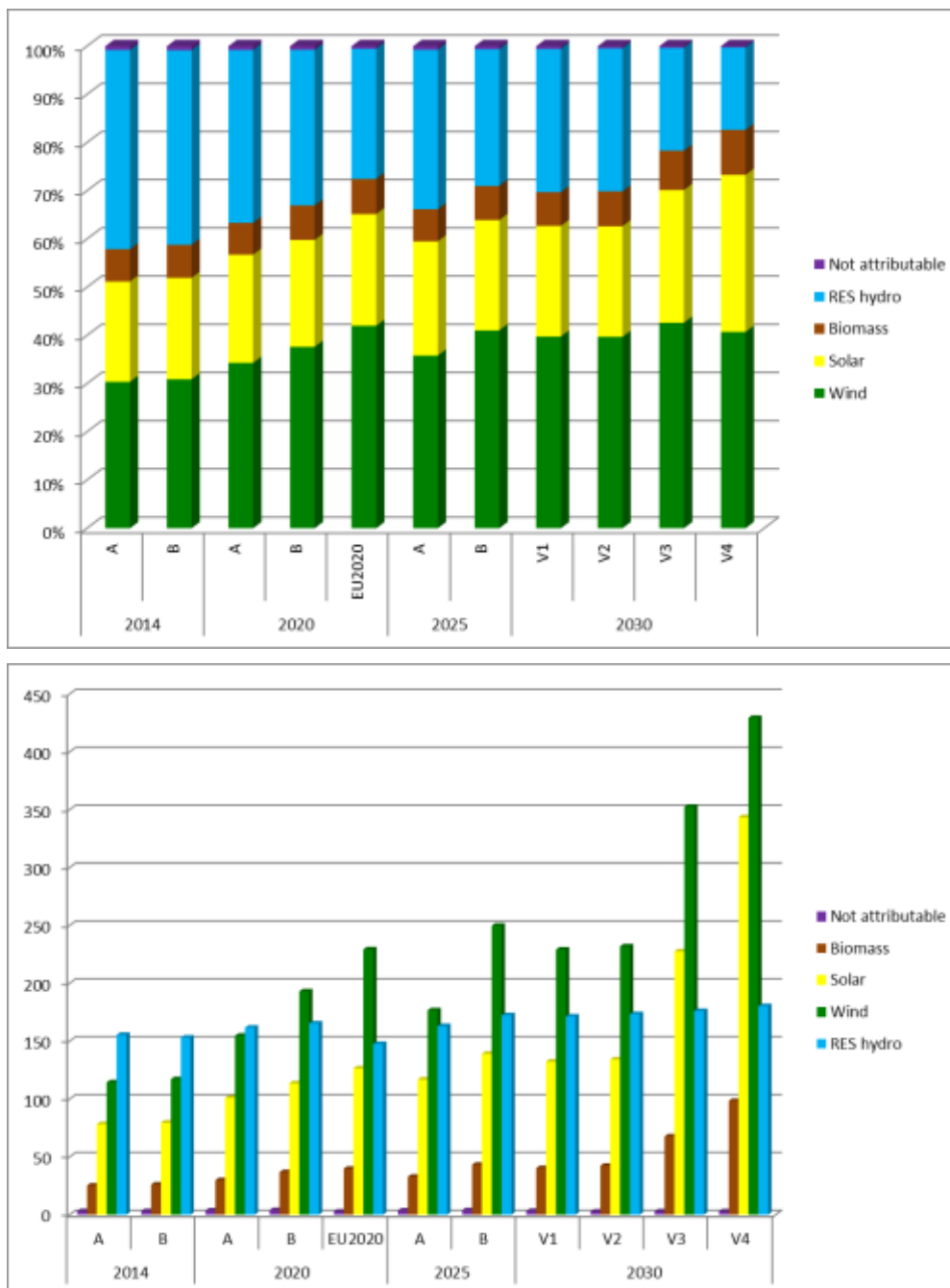
F. 3.2.4.3 – ENTSO-E RES generation capacity breakdown; all scenarios; January 7 p.m.
