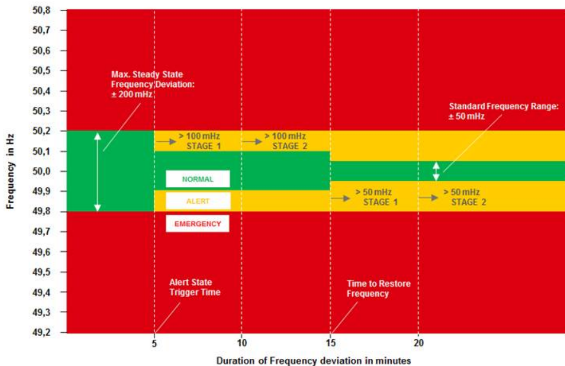
Figure 8: Illustration of Stage 1 and Stage 2 based on the System States of the SO GL 10 .
