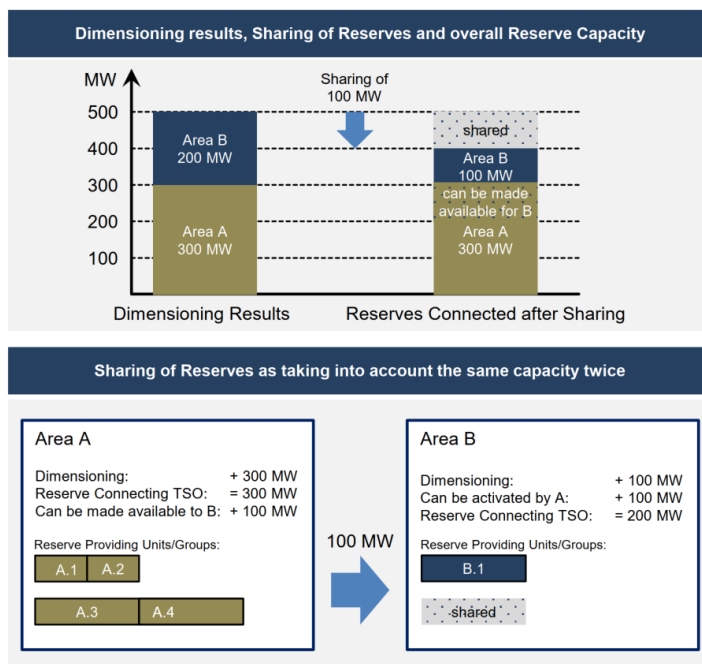
Figure 2: Sharing of reserve capacity – simple example
