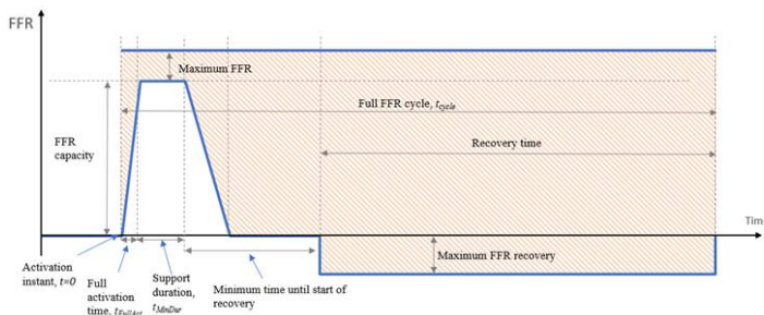
Figure 3: Sequential diagram for the activation of FFR
