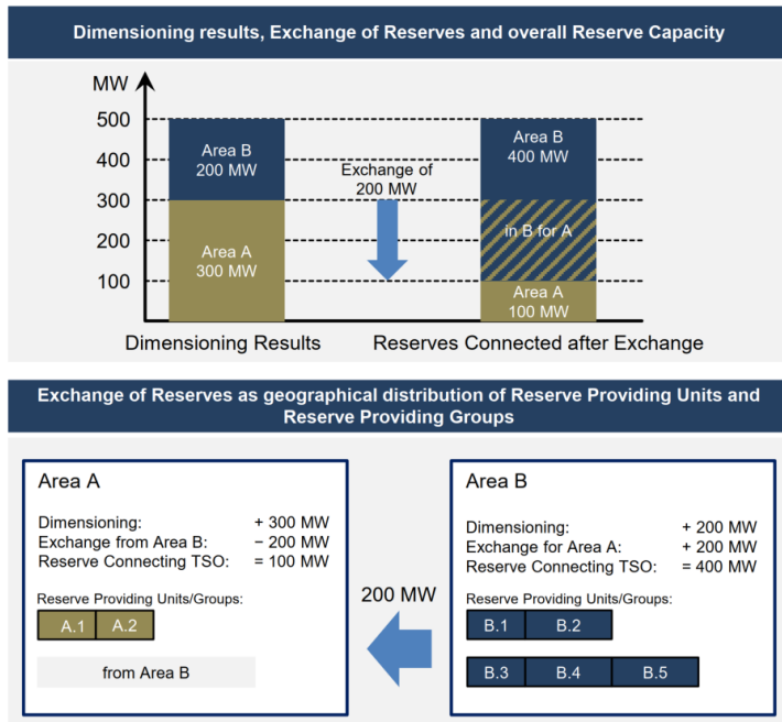
Figure 1: Exchange of reserve capacity – simple example
