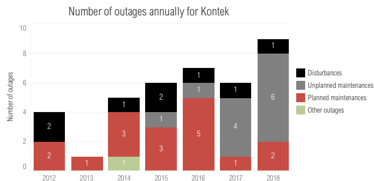
Figure 5.30: The annual number of disturbances, unplanned and planned maintenance outages and other outages Kontek for the years 2012–2018.
