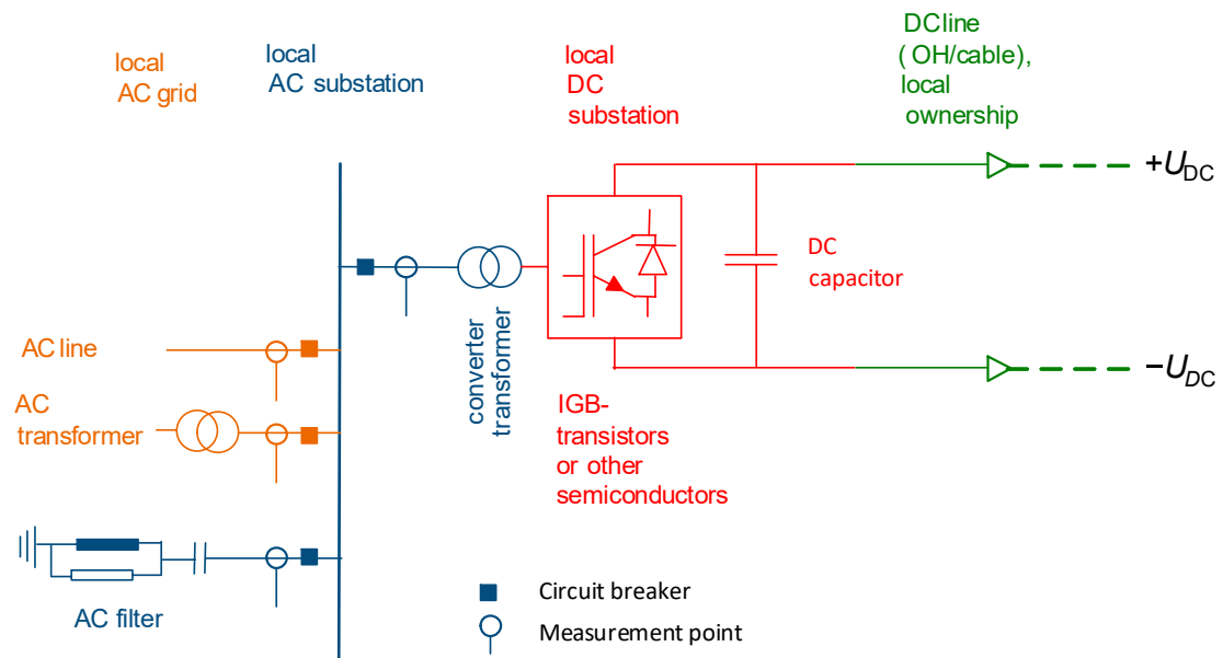
Figure A.3: A schematic presentation of an HVDC link with voltage source converters (VSC)
