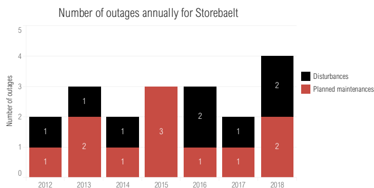
Figure 5.70: The annual number of disturbances, unplanned and planned maintenance outages and other outages Storebælt for the years 2012–2018. Storebælt had no other outages during the years 2012–2018.
