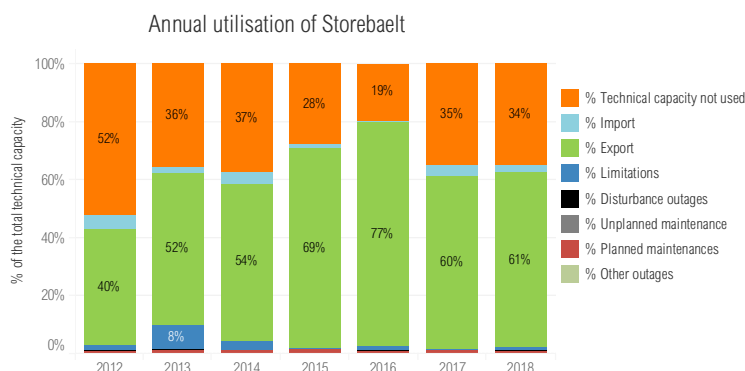
Figure 5.68: Annual utilisation of Storebælt according to the utilisation and unavailability categories for the years 2012–2018. The utilisation and unavailability categories are described in more detail in Section 3.
